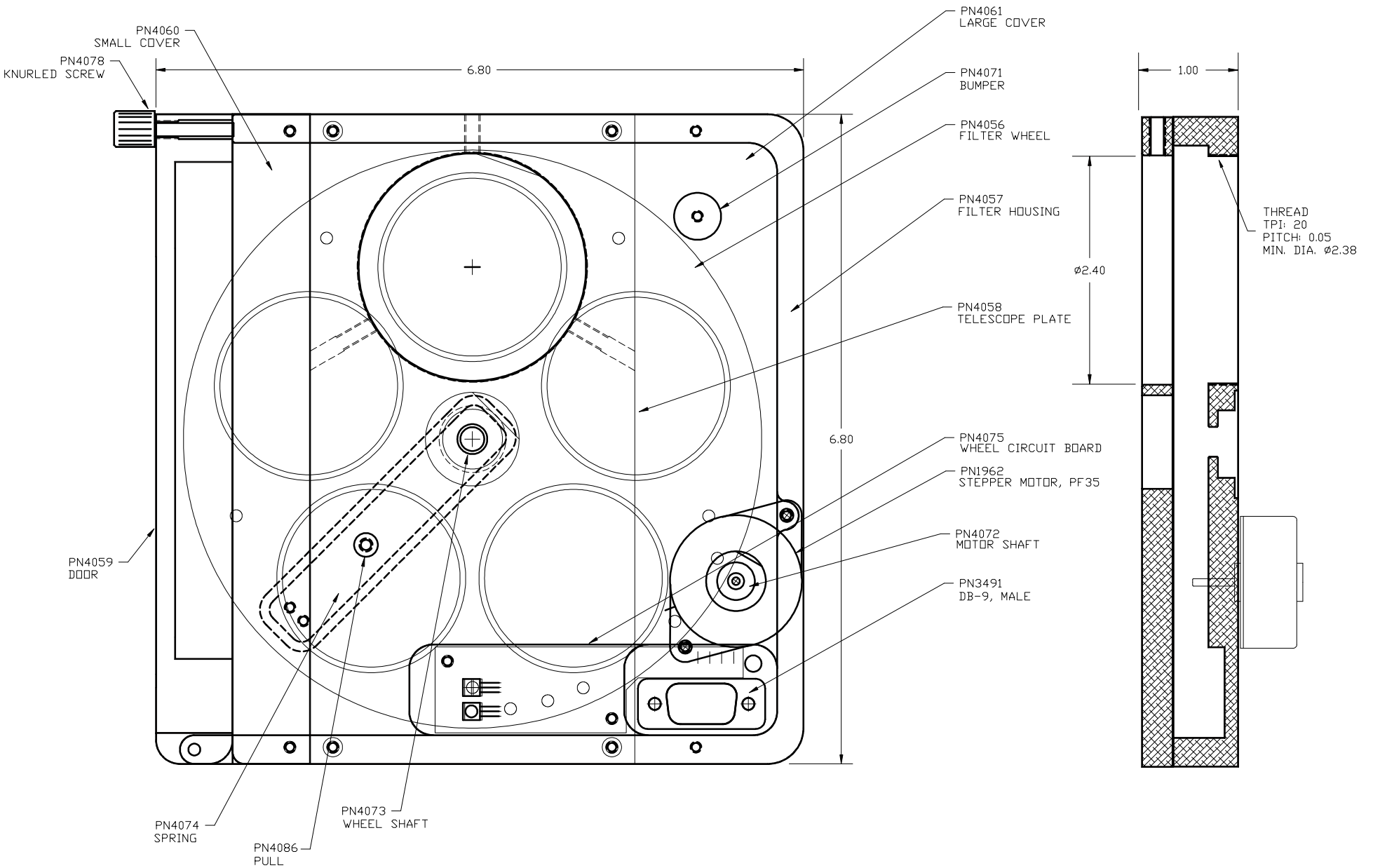
VIEW FROM TELESCOPE TOWARD EYEPIECE OR CAMERA
