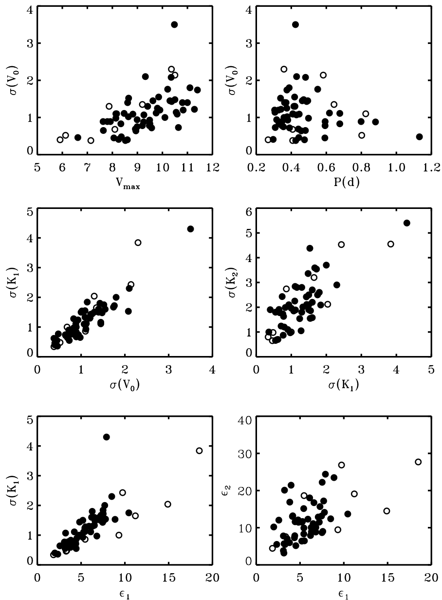
FIG. 4.—Correlations between various mean standard errors as given in the axis labels. Top : \sigma(V_0) as a function of V_{\max} and the orbital period, P . \sigma(V_0) is a convenient measure of the solution quality and correlates tightly with \sigma(K_1) , as shown in the middle left panel. The middle right panel shows the correlation between \sigma(K_1) and \sigma(K_2) . This correlation is not perfect because of the very large range of mass ratios observed among binaries of this program. The two bottom panels show the errors per observation \epsilon ; the left panel shows the correlation between \epsilon_1 and \sigma(K_1) , while the right panel shows the correlation between \epsilon_1 and \epsilon_2 . In all panels binaries analyzed through subtraction of the third-component signatures from the broadening functions are marked by open circles. All quantities are expressed in kilometers per second.
